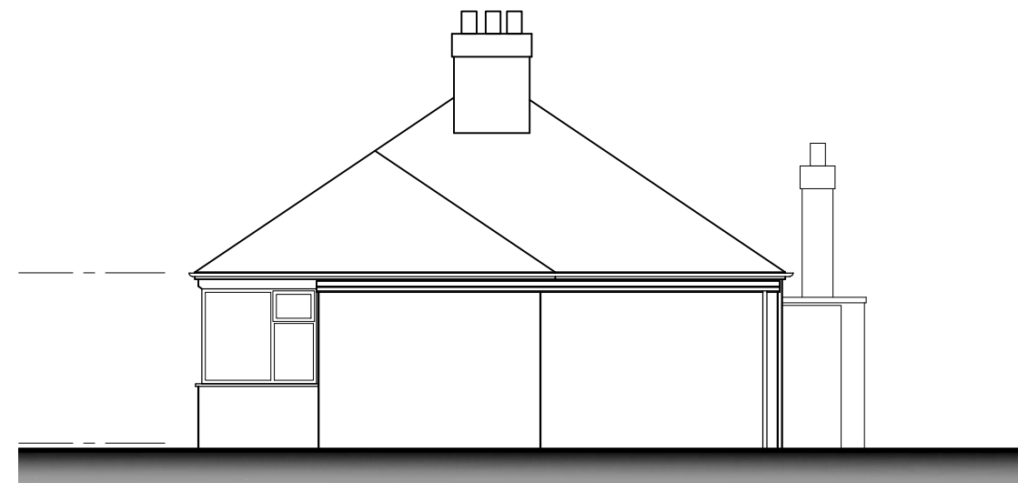
Side Elevation @ 1:100
